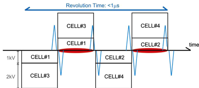
FIG. 33. In the third stage ( T_r < 1\ \mu\text{s} ), two pairs of type A and B ICs are operated intermittently.
