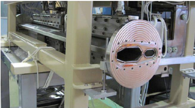
FIG. 23. Septum magnet and new vacuum ducts. The left duct is for the circulating beam and the right duct is for the extracted beam.
