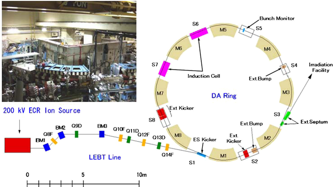
FIG. 2. Outline of the KEK digital accelerator and the recent photograph.
