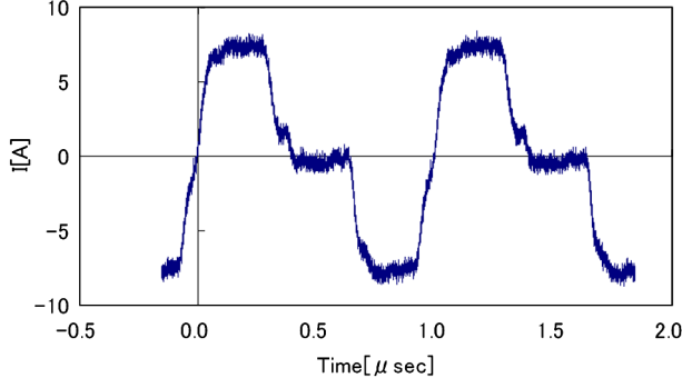
FIG. 40. Output current observed at the matching resistor of the acceleration cell.
