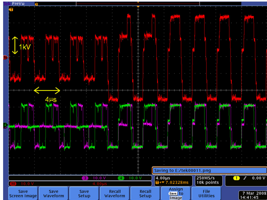
FIG. 39. Output voltage waveform at the transition between stages 1 and 2. (Voltage and time scales are indicated by double-headed arrows.)
