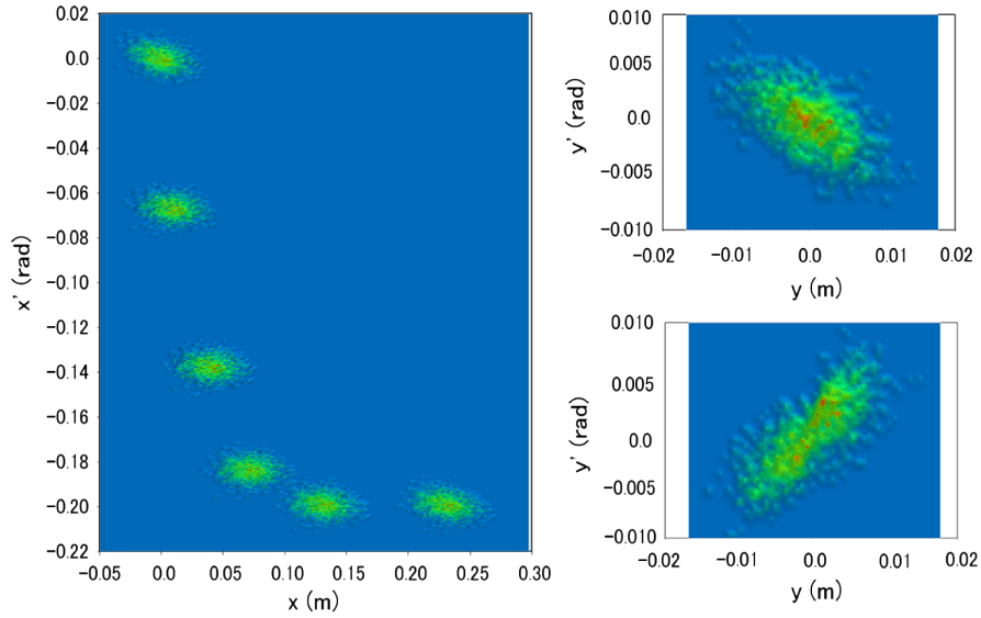
FIG. 19. Phase space distribution in the kicker field. In the left figure, the phase plot moves from the lower right to the upper left along the beam passage. The origin corresponds to the end of the injection kicker. Two right-hand figures show the beam distributions in the vertical phase space: the upper figure is for the beam at the entrance and the lower is at the exit of the kicker. The central orbit in the DA ring is x = 0.0 and y = 0.0 in each figure.
