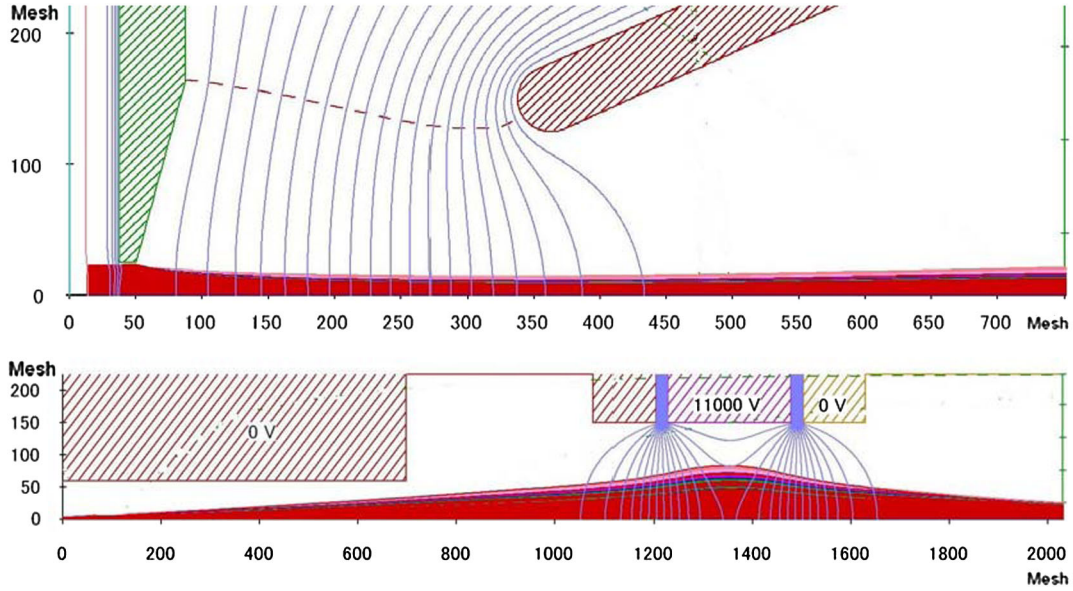
FIG. 5. Beam envelope from cathode to anode and from anode through Einzel lens (IGUN simulation result). Units are mesh size in simulation ( 20 \mu\text{m} in this calculation).
