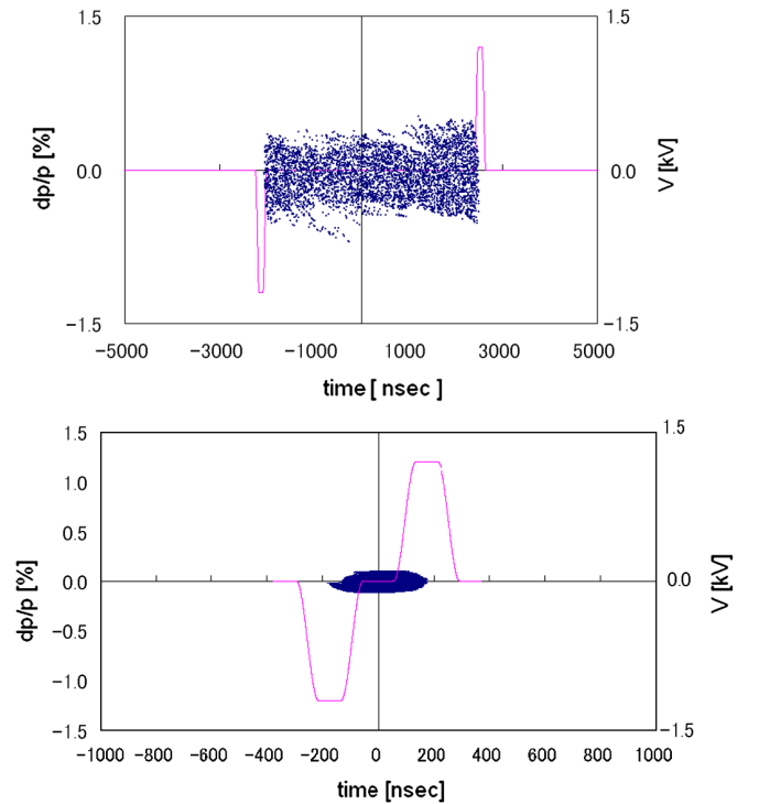
FIG. 34. Phase plot of an \text{Ar}^{8+} beam 100 turns after injection (top) and just before extraction (bottom). Dots show injected ions and the purple lines correspond to barrier voltages for confinement (unit: kV).
