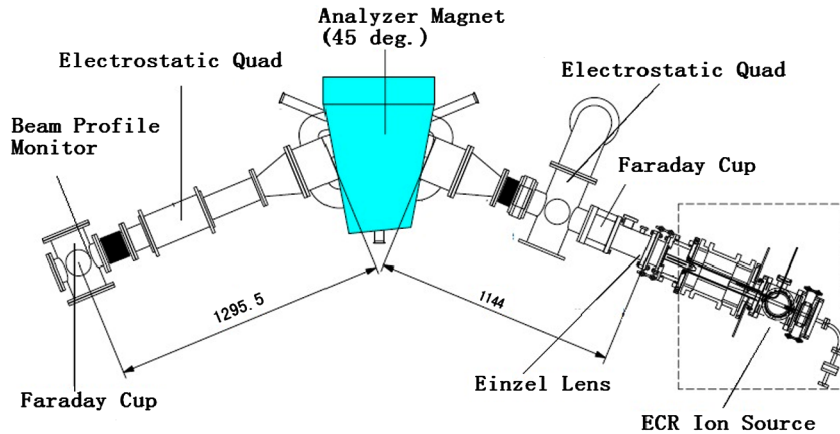
FIG. 6. Schematic overview of the test bench (unit is mm).
