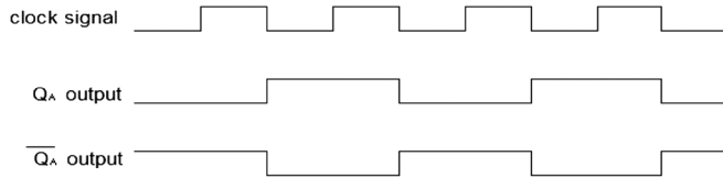
FIG. 38. In the third stage, the signal divider generates gate triggers Q_A and \bar{Q}_A for two sets of ICs.
