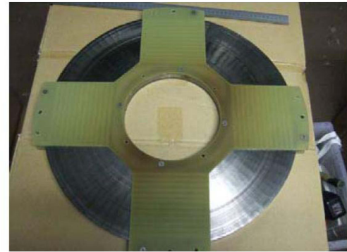
FIG. 29. Inner structure of an IC (top) and a magnetic core bobbin and G-10 spacer with oil flow channels (bottom).
