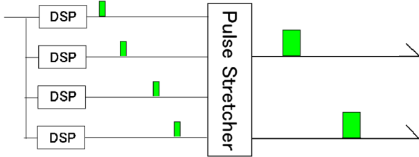
FIG. 37. Pulse stretcher generates set/reset pulse signals with widths that can be controlled by the separations of the input pulses.
