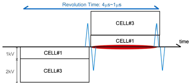
FIG. 32. In the second stage ( 1\ \mu\text{s} < T_r < 2\ \mu\text{s} ), a type A and a type B IC are triggered simultaneously.
