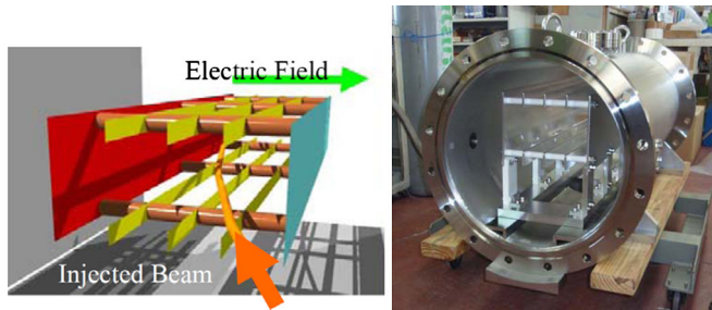
FIG. 16. Schematic view of the injection kicker (left) and a photograph of the kicker (right).
