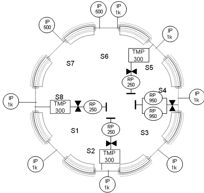
FIG. 26. Overview of the DA ring vacuum system. RP, TMP, and IP denote a rotary pump, turbo molecular pump, and ion getter pump, respectively. The numbers after the pump type are their pumping speed (l/min).
