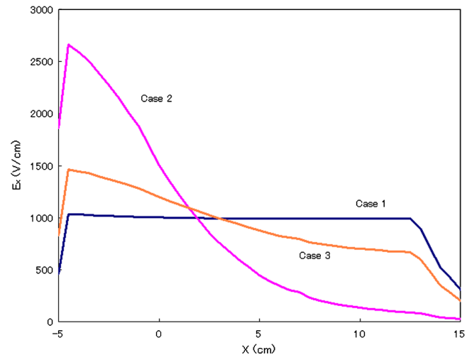
FIG. 18. Horizontal component of the electric field E_x at the center of the kicker electrode ( y = z = 0 ) vs x . In case 1 the subsidiary electrodes share the voltage equally. In case 2 each subsidiary electrode is floated. In case 3 all subsidiary electrodes are removed.
