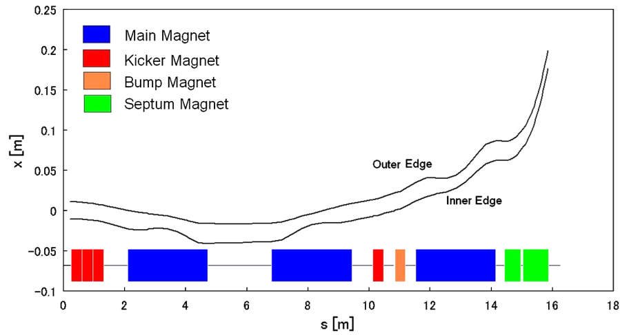
FIG. 22. Extraction system and the beam envelope.
