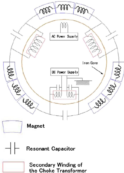
FIG. 14. Resonant network for excitation of KEK-DA main magnets.
