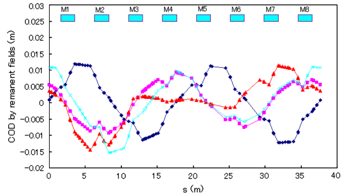
FIG. 42. CODs calculated from the remanent field. Squares at the top of the figure indicate the positions of the eight magnets. Each of the four lines corresponds to one of the cases described in Sec. VIII B.
