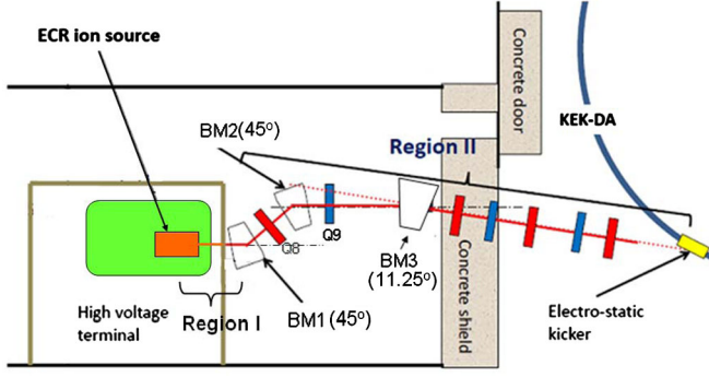
FIG. 10. LEPT line from the ECRIS to the DA ring.
