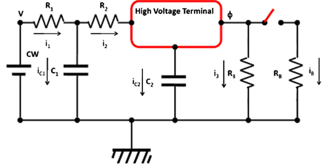
FIG. 9. Equivalent circuit of the HVT used to estimate voltage stability. R_1 and R_2 are the resistances of feeder line. R_3 is the resistance of the ceramic chamber. R_B is the resistance seen by the beam current. C_1 is a capacitance inserted to stabilize the voltage. C_2 is the stray capacitance of the HVT.
