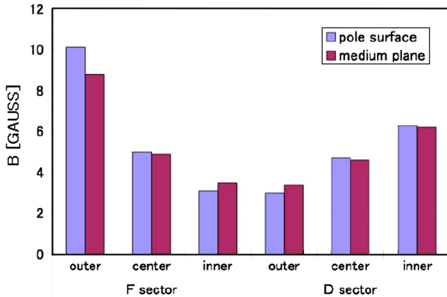
FIG. 41. Measured remanent field of the monitor magnet.
