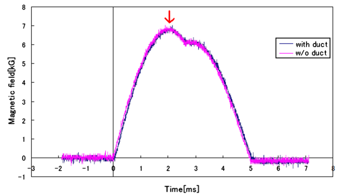
FIG. 24. Time profile of the septum magnetic fields. The arrow indicates the extraction timing.
