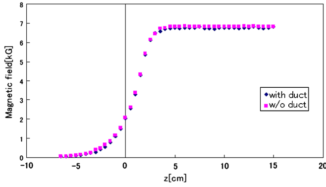
FIG. 25. Peak fields of the septum magnet along the beam axis.
