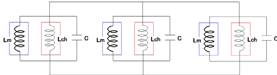
FIG. 15. Equivalent circuit for the resonant network.
