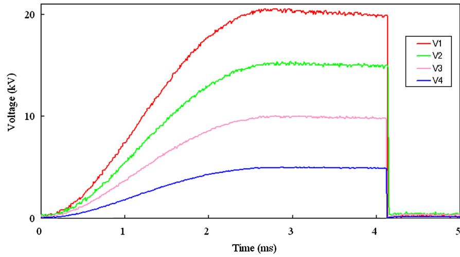
FIG. 21. Voltage waveforms measured at kicker electrodes. Voltages V1–V4 correspond to the voltages at the anode and the subsidiary electrodes S1–S3, respectively.
