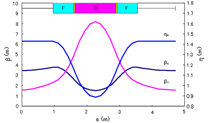
FIG. 12. Beta functions and dispersion function.
