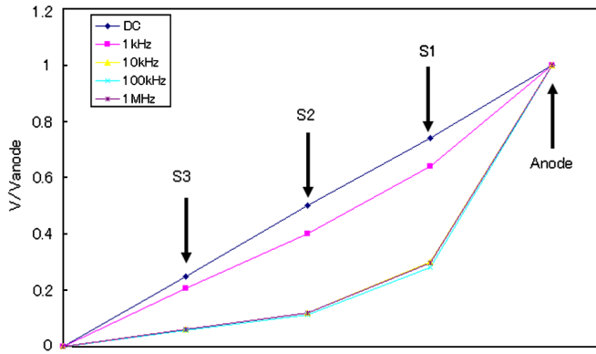
FIG. 20. Voltages measured at the anode and subsidiary electrodes S1, S2, and S3 (normalized by the anode voltage).
