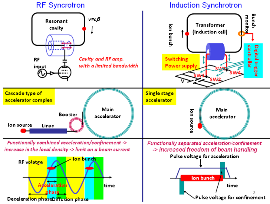
FIG. 1. Comparison between an rf synchrotron and an induction synchrotron (digital accelerator).
