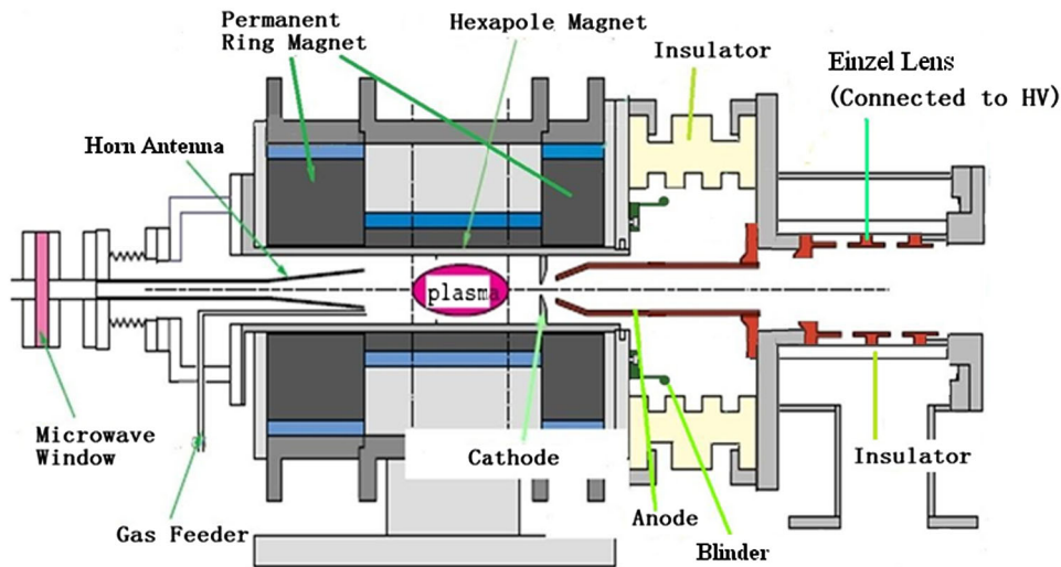
FIG. 3. Outline of ECRIS with the extraction system downstream.
