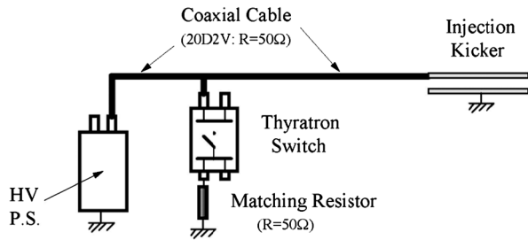
FIG. 17. Pulse forming network for the injection kicker.
