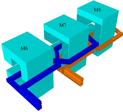
FIG. 44. Two sets of figure-eight back-leg coils for COD correction.
