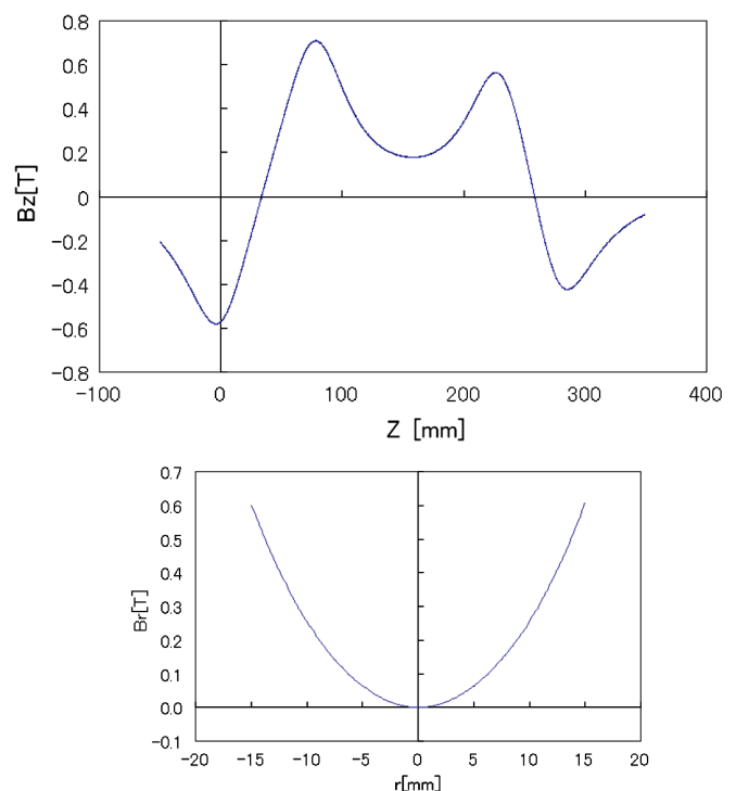
FIG. 4. Field distribution measured through the ECRIS, (top) B_z(z) and (bottom) B_r(r) at the minimum B_z .
