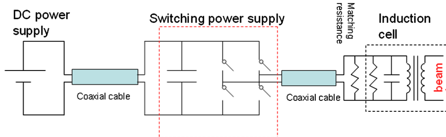
FIG. 27. An equivalent circuit for the induction acceleration system.
