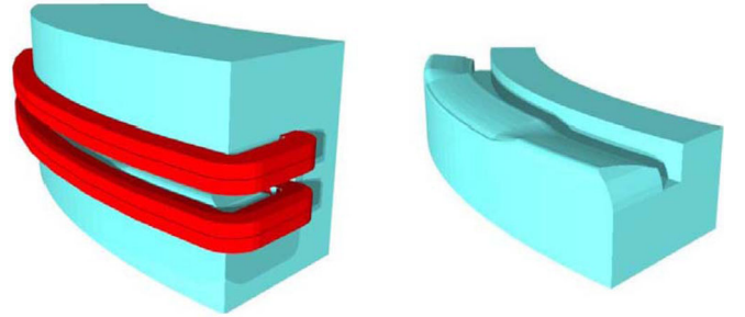
FIG. 13. Schematic view of the main magnet. In the right-hand figure, the upper half of the magnet core is omitted to show the pole shape.
