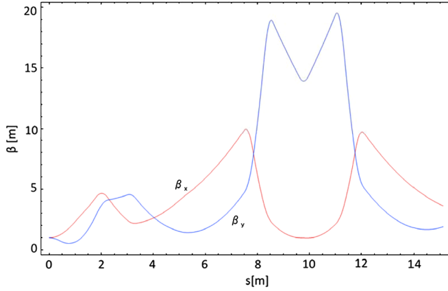
FIG. 11. Beta functions in the x and y directions.
