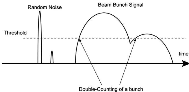
FIG. 35. Difficulties in obtaining beam bunch timing by setting a fixed threshold.
