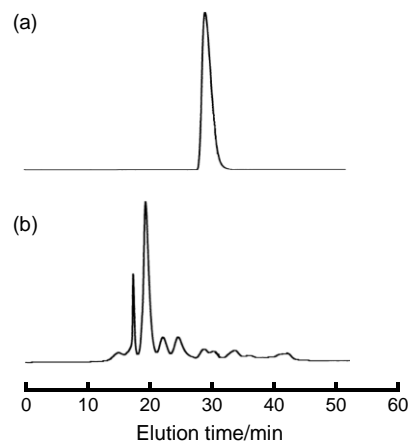
Fig. 6 HPLC charts of (a) 2b(O) and (b) the colourless solution after the thermal bleaching reaction of a photostationary solution of 2b upon irradiation with UV light at -60 °C. The peak intensity was detected by absorbance at 254 nm in hexane/ethyl acetate (98:2).
