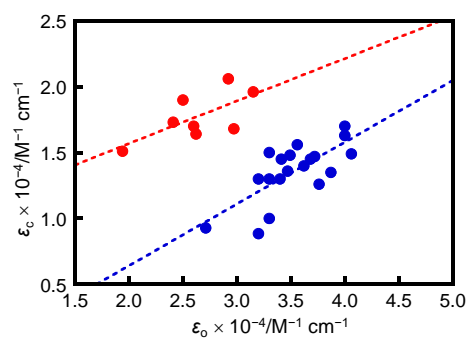
Fig. 3 Relationship between the molar absorption coefficients of the open-ring isomer ( \epsilon_o ) and the closed-ring isomer ( \epsilon_c ) for diarylethenes ( \bullet : R^2 = 0.517 ) and thiophene- S,S -dioxidized diarylethenes ( \bullet : R^2 = 0.447 ) reported previously. 18,20
