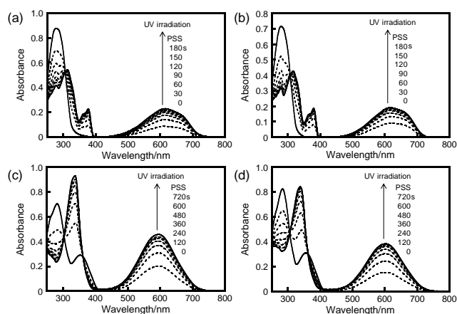
Fig. 2 Absorption spectral changes of (a) 1a , (b) 2a , (c) 1b and (d) 2b in n -hexane upon irradiation with 313 nm light at -60\text{ }^{\circ}\text{C} : [ 1a ] = 2.03 \times 10^{-5}\text{ M} , [ 2a ] = 1.44 \times 10^{-5}\text{ M} , [ 1b ] = 2.40 \times 10^{-5}\text{ M} and [ 2b ] = 2.62 \times 10^{-5}\text{ M} , respectively.
