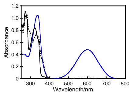
Fig. 5 Absorption spectra of the photostationary solution of 2b at -60 °C (blue solid line), the solution after the thermal bleaching reaction (black solid line) and the UV irradiated solution after the thermal bleaching reaction (black dashed line).
