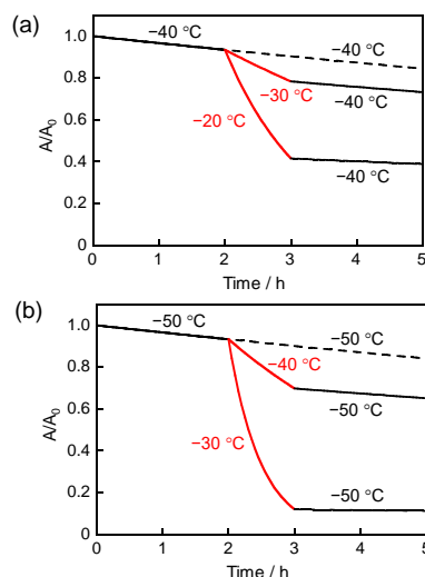
Fig. 7 Calculated absorbance changes of (a) 1b(C) and (b) 2b(C) in n -hexane stored for 5 h at -40 or -50 °C (---) and heated up for 1 h on the way (—).
