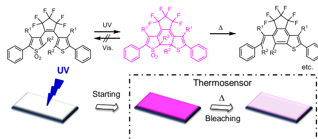
Fig. 1 Concept of light-starting irreversible thermosensors using thiophene- S,S -dioxidized diarylethenes
